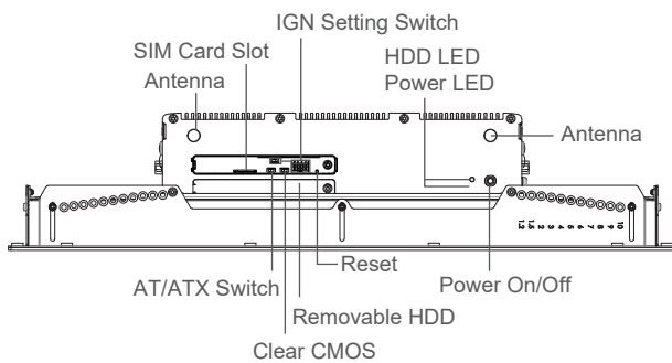
Front I/O
