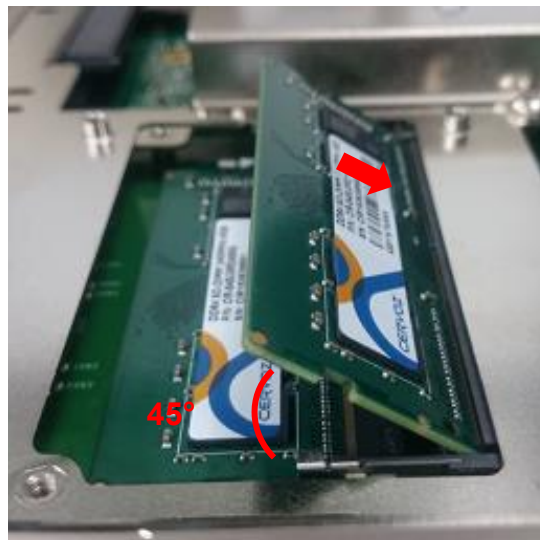
Upper socket
