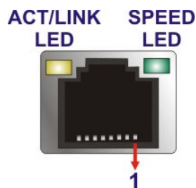
Figure 3-25: Ethernet Connector
