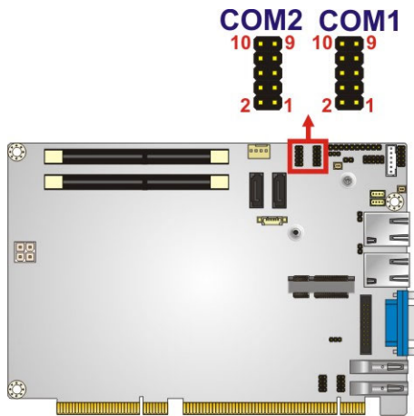
Figure 3-19: RS-232/422/485 Serial Port Connector Locations
