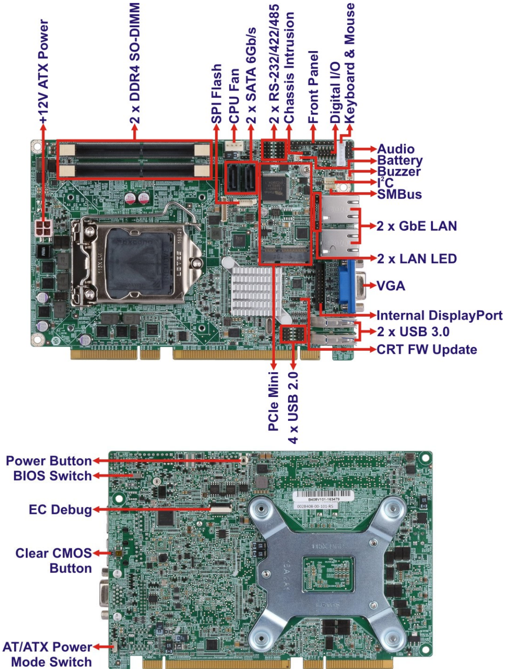
Figure 1-2: Connectors
