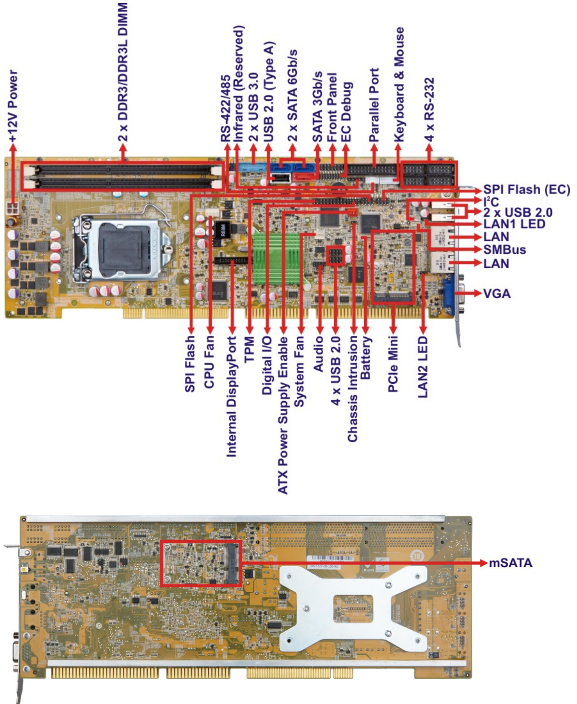
Figure 1-2: Connectors
