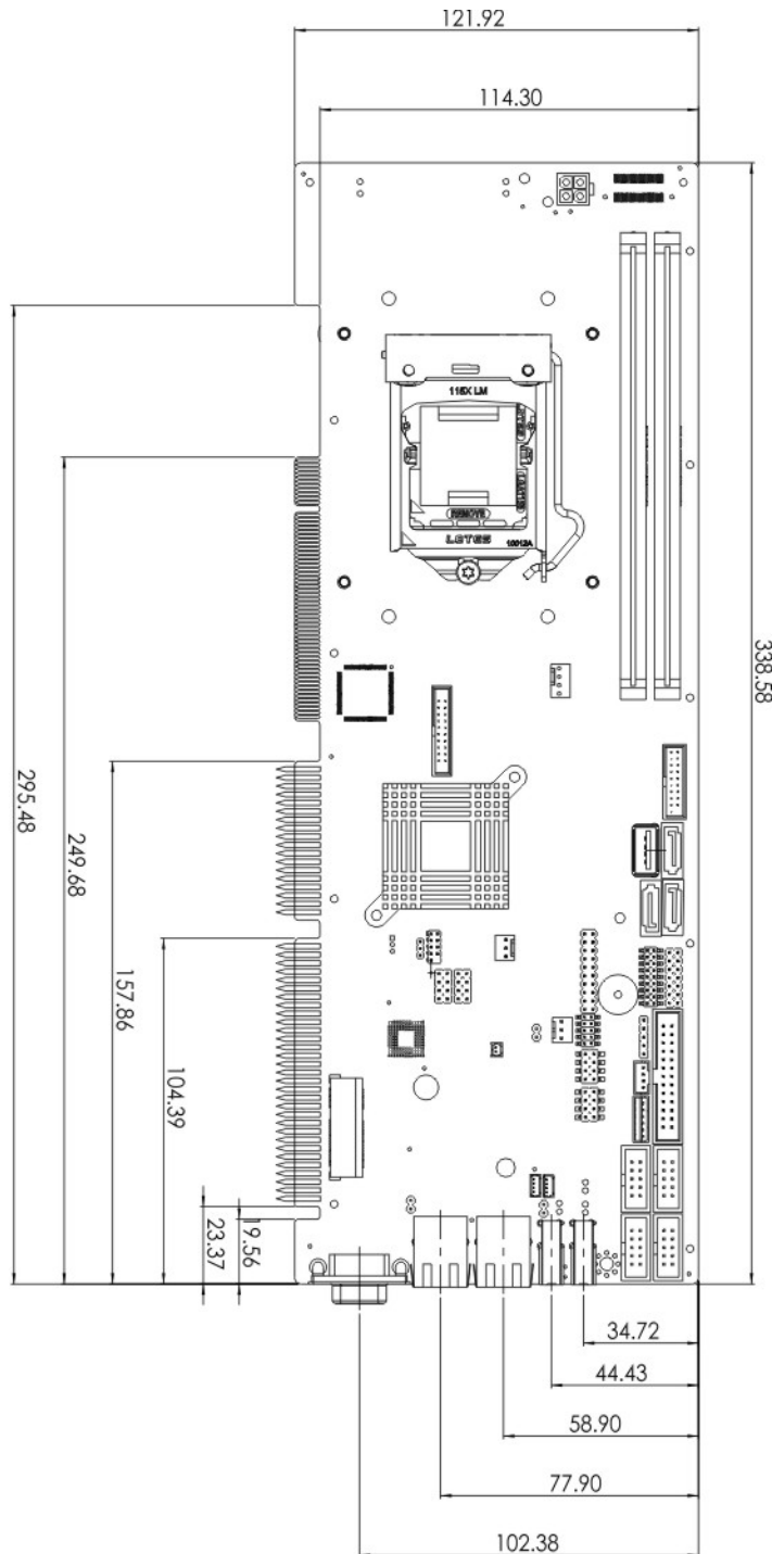
Figure 1-3: WSB-H810 Dimensions (mm)
