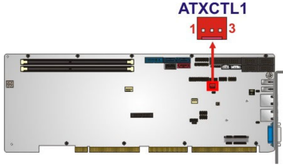
Figure 3-3: ATX Power Supply Enable Connector Location
