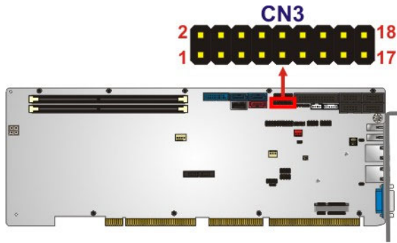
Figure 3-9: EC Debug Connector Location
