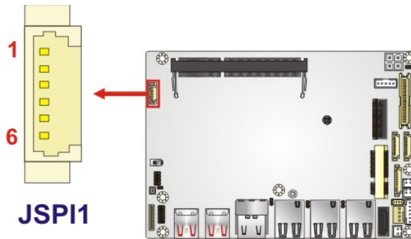
Figure 3-21: SPI Flash Connector Location
