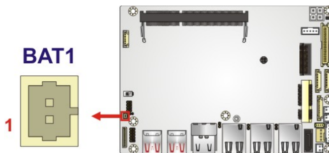
Figure 3-3: Battery Connector Location
