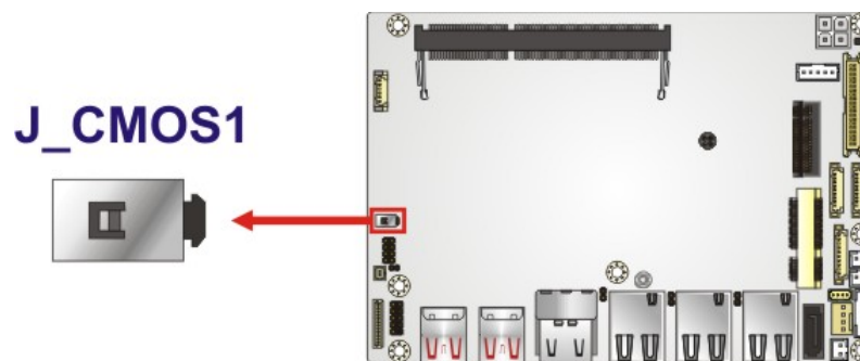
Figure 4-8: Clear CMOS Button Location
