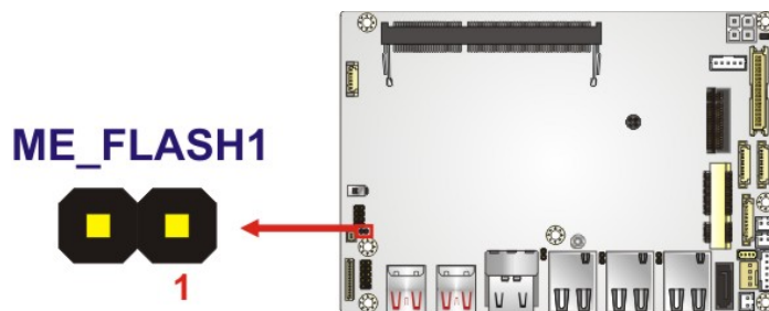
Figure 4-9: Flash Descriptor Security Override Jumper Location
