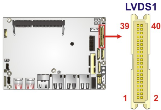
Figure 3-8: LVDS Connector Location
