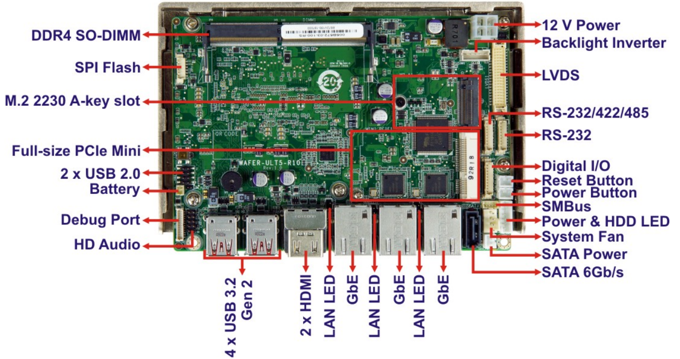
Figure 1-2: Connectors
