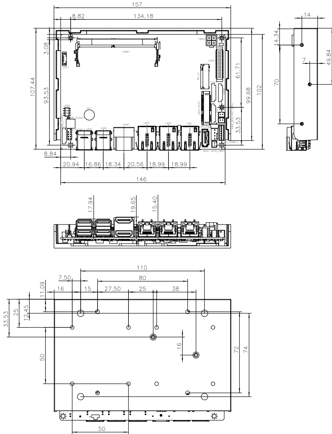
Figure 1-3: Dimensions (mm)
