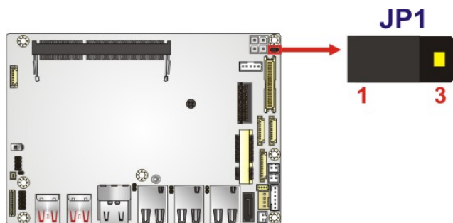
Figure 4-10: LCD Voltage Selection Jumper Location
