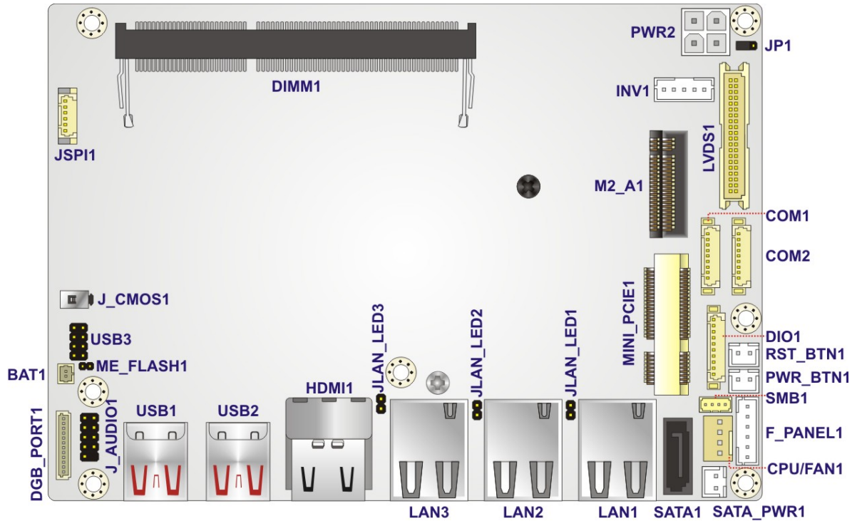
Figure 3-1: Connector and Jumper Locations
