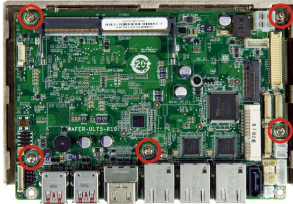
Figure 4-11: Heat Sink Retention Screws
