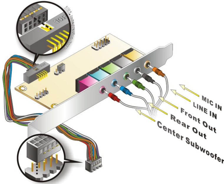
Figure 4-15: 7.1 Channel Audio Kit
