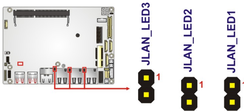
Figure 3-7: LAN LED Connector Locations
