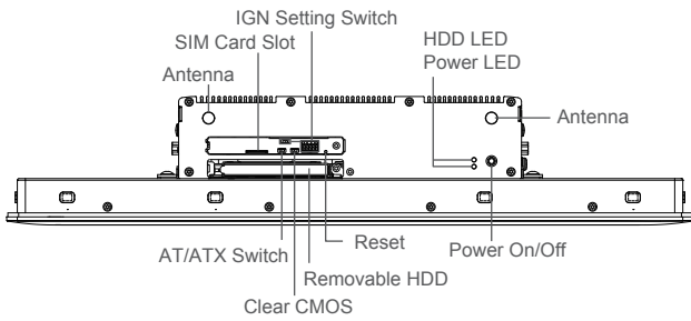
Front I/O
