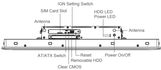
Front I/O
