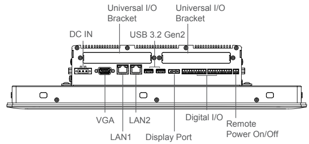
Rear I/O
