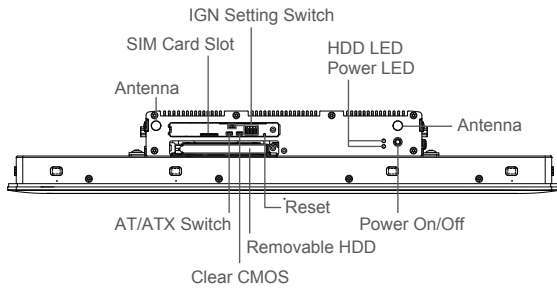
Front I/O
