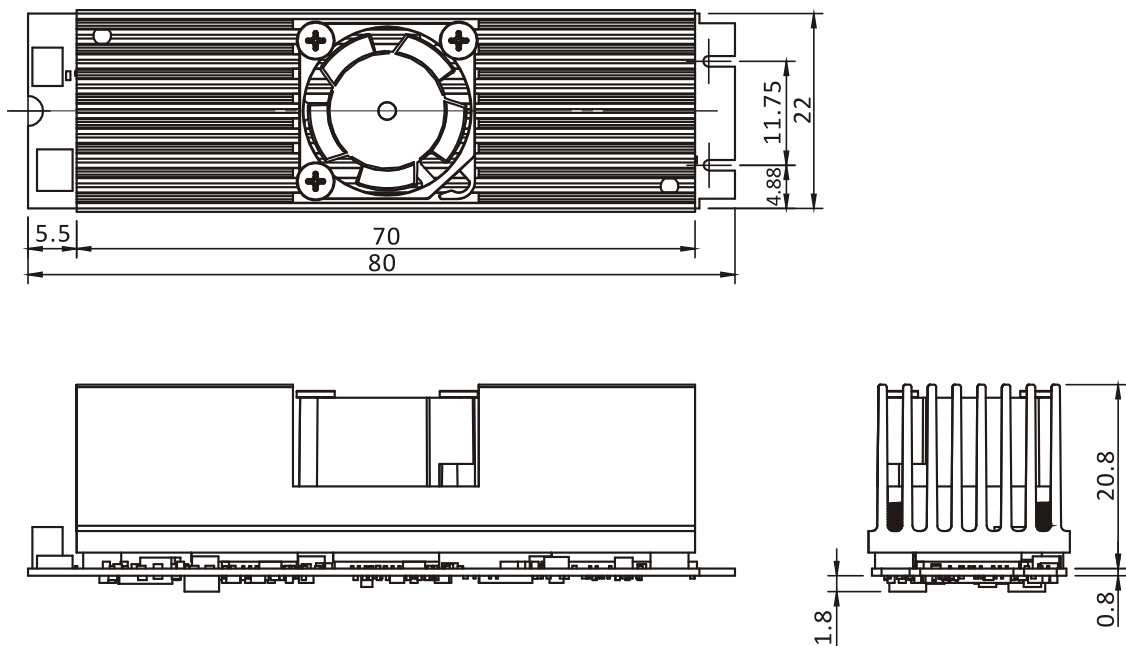
Figure 1-2: Dimensions (mm)
