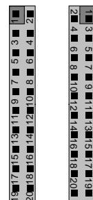
I²C Digital I/O X50 X51
