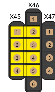
SPI Jumper
