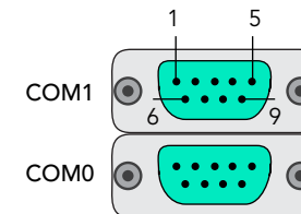
COM Ports - Connector X41
