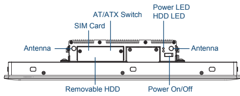
Front I/O
