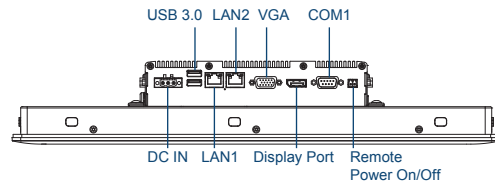
Rear I/O
