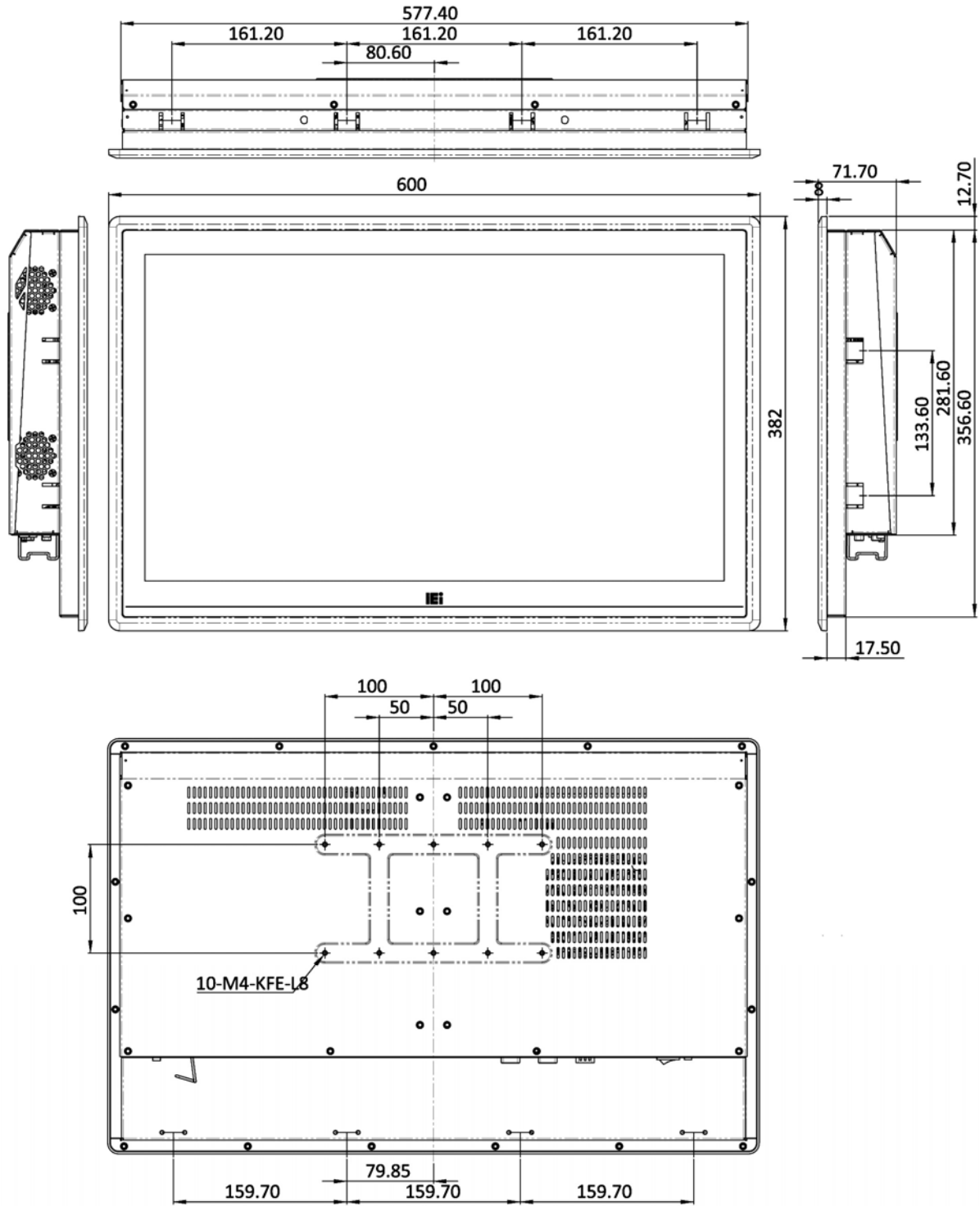
Figure 1-10: PPC-F24A-H81 Dimensions (mm)
