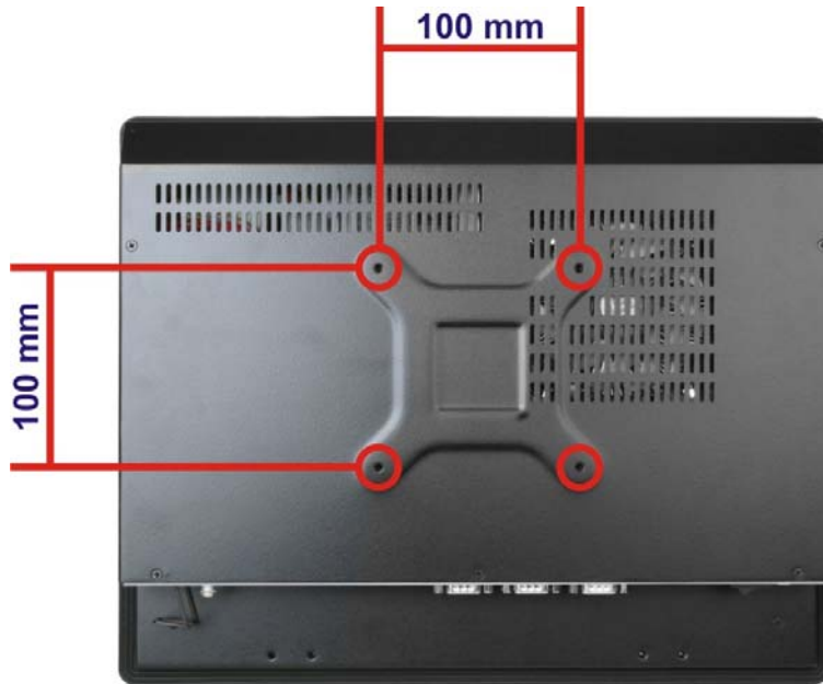
Figure 3-32: Stand Mounting Retention Screw Holes
