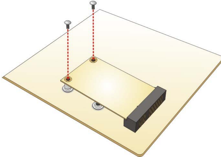
Figure 3-15: Securing the PCIe Mini Card
