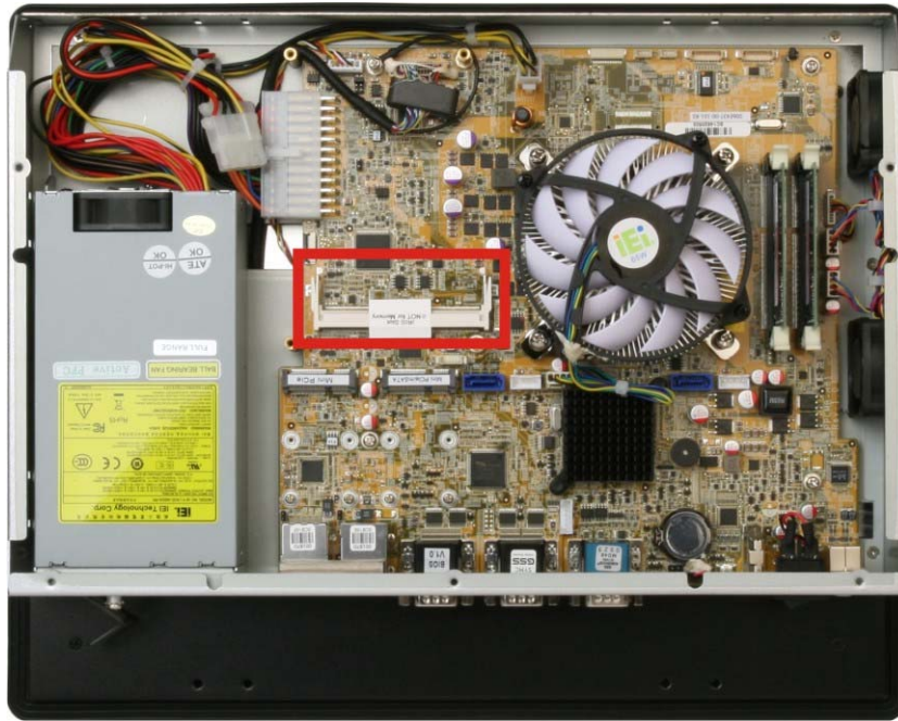
Figure 3-16: iRIS-2400 Module Slot
